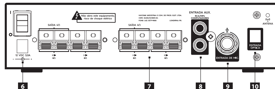
Painel Traseiro
